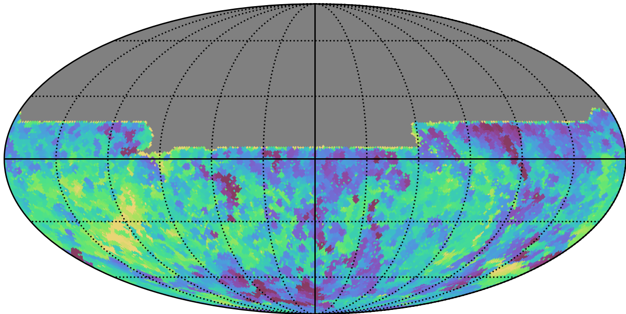
noroll_mjdp0_v3.4_10yrs All sky y band: Min fiveSigmaDepth
