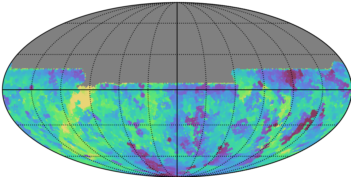
noroll_mjdp0_v3.4_10yrs All sky u band: Min fiveSigmaDepth
