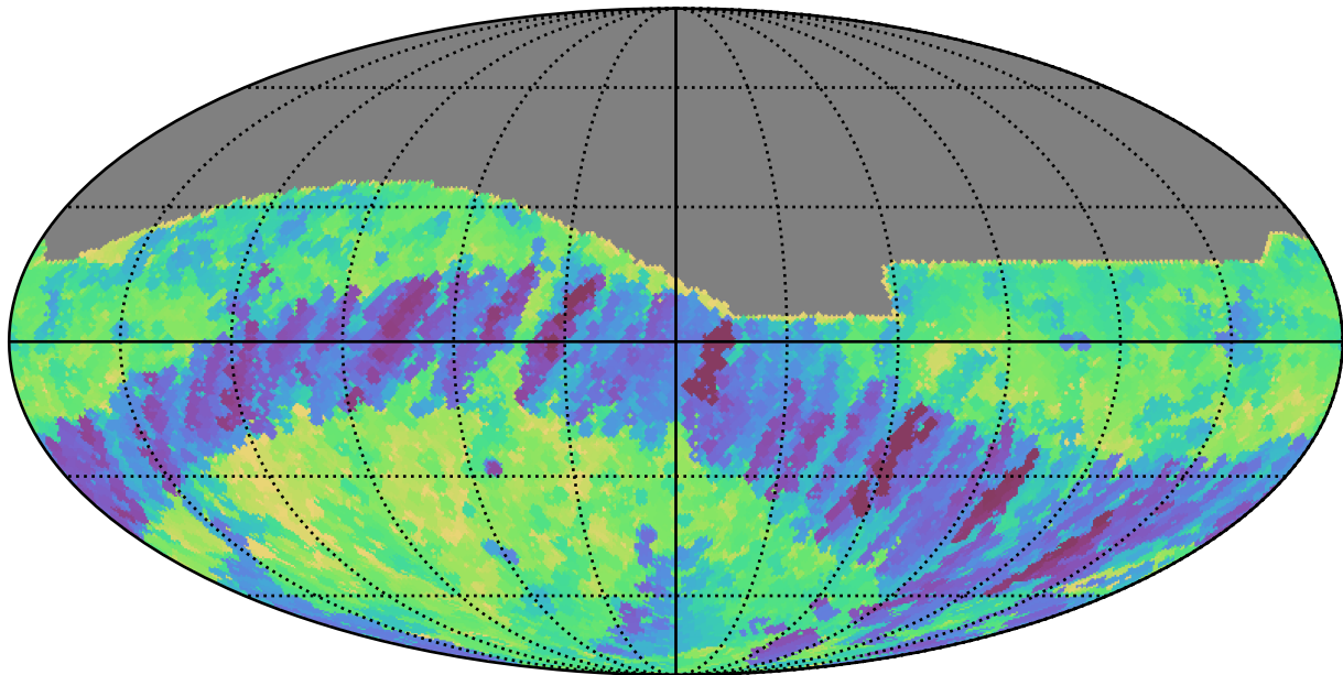
noroll_mjdp0_v3.4_10yrs All sky r band: Min fiveSigmaDepth
