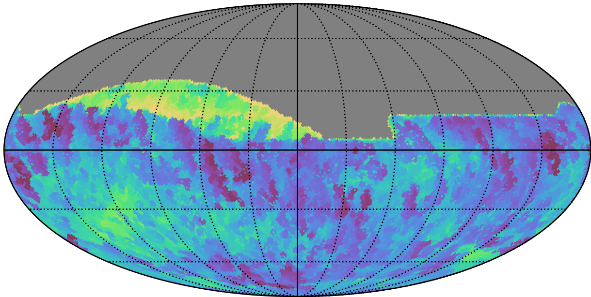
noroll_mjdp0_v3.4_10yrs All sky all bands: Min fiveSigmaDepth
