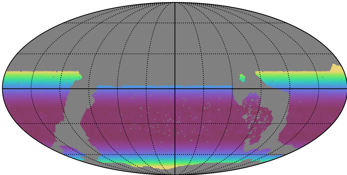
noroll_mjdp0_v3.4_10yrs WFD z band: Min airmass
