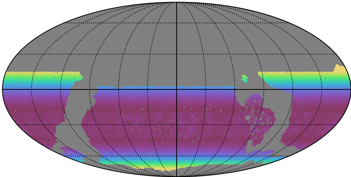
noroll_mjdp0_v3.4_10yrs WFD u band: Min airmass
