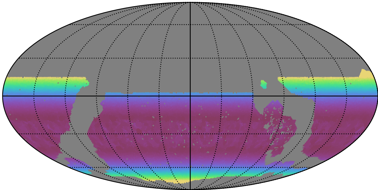
noroll_mjdp0_v3.4_10yrs WFD g band: Min airmass
