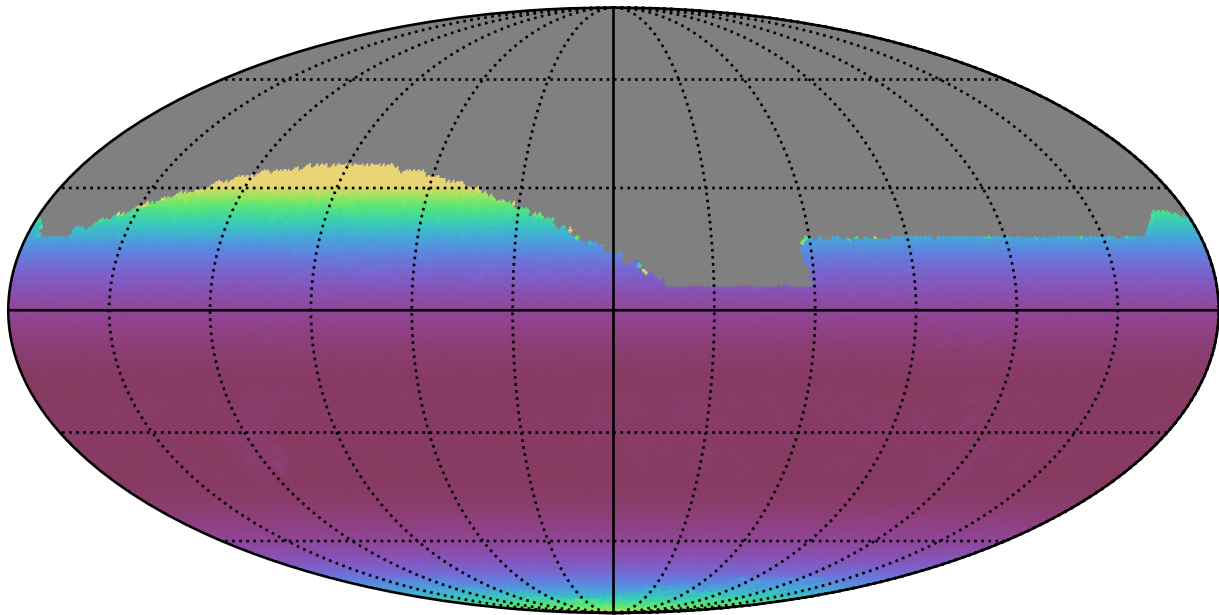
noroll_mjdp0_v3.4_10yrs All sky z band: Min airmass
