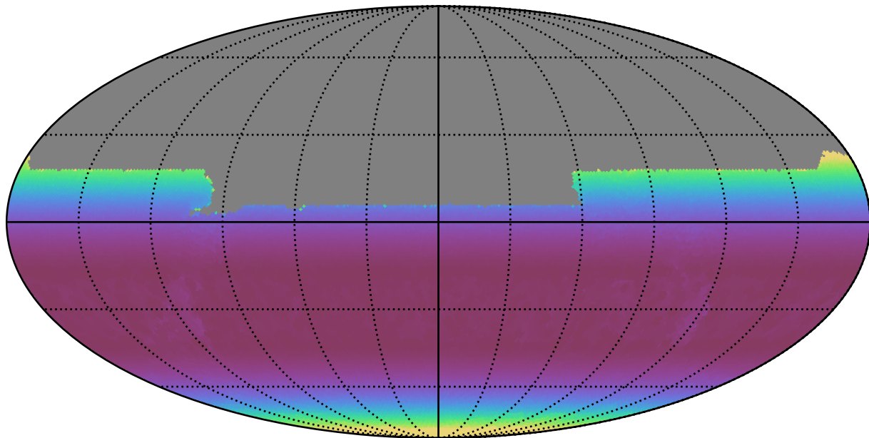
noroll_mjdp0_v3.4_10yrs All sky y band: Min airmass
