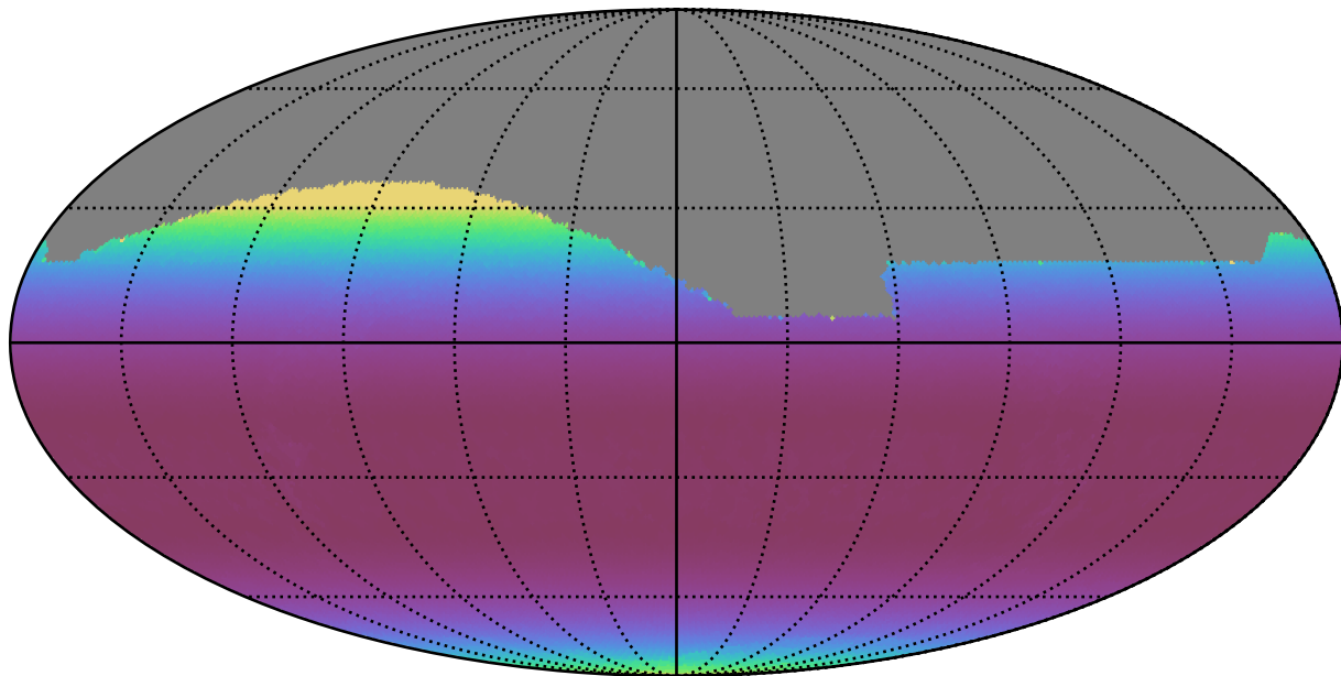
noroll_mjdp0_v3.4_10yrs All sky i band: Min airmass
