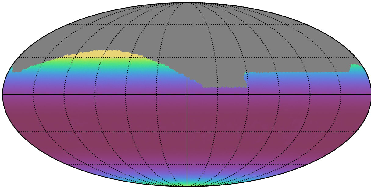
noroll_mjdp0_v3.4_10yrs All sky all bands: Min airmass
