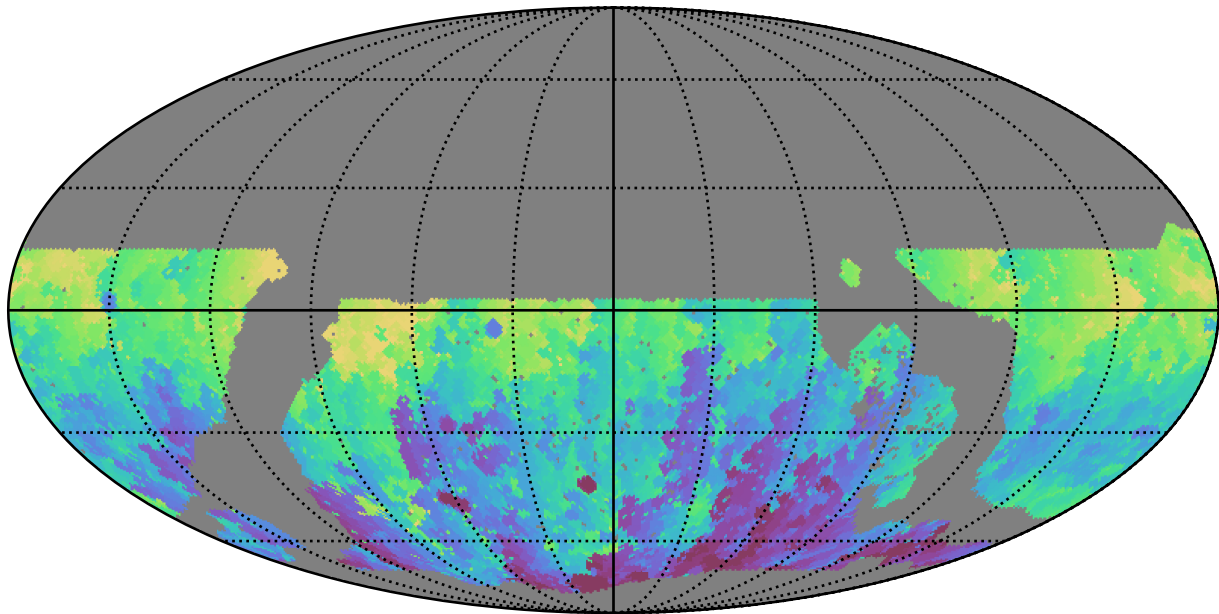
noroll_mjdp0_v3.4_10yrs WFD u band: Min HA
