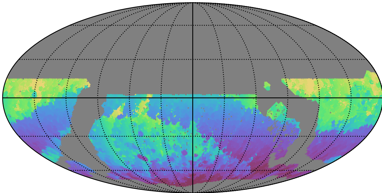
noroll_mjdp0_v3.4_10yrs WFD r band: Min HA
