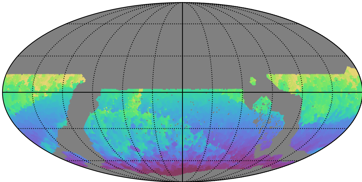
noroll_mjdp0_v3.4_10yrs WFD all bands: Min HA
