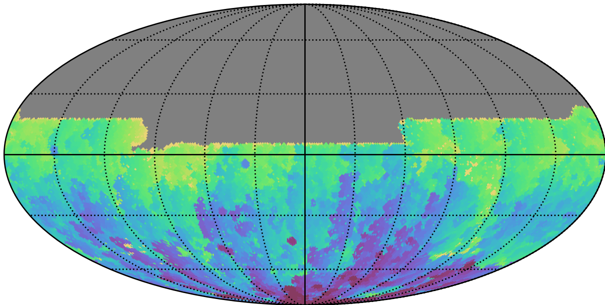
noroll_mjdp0_v3.4_10yrs All sky u band: Min HA
