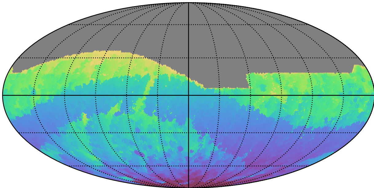
noroll_mjdp0_v3.4_10yrs All sky r band: Min HA
