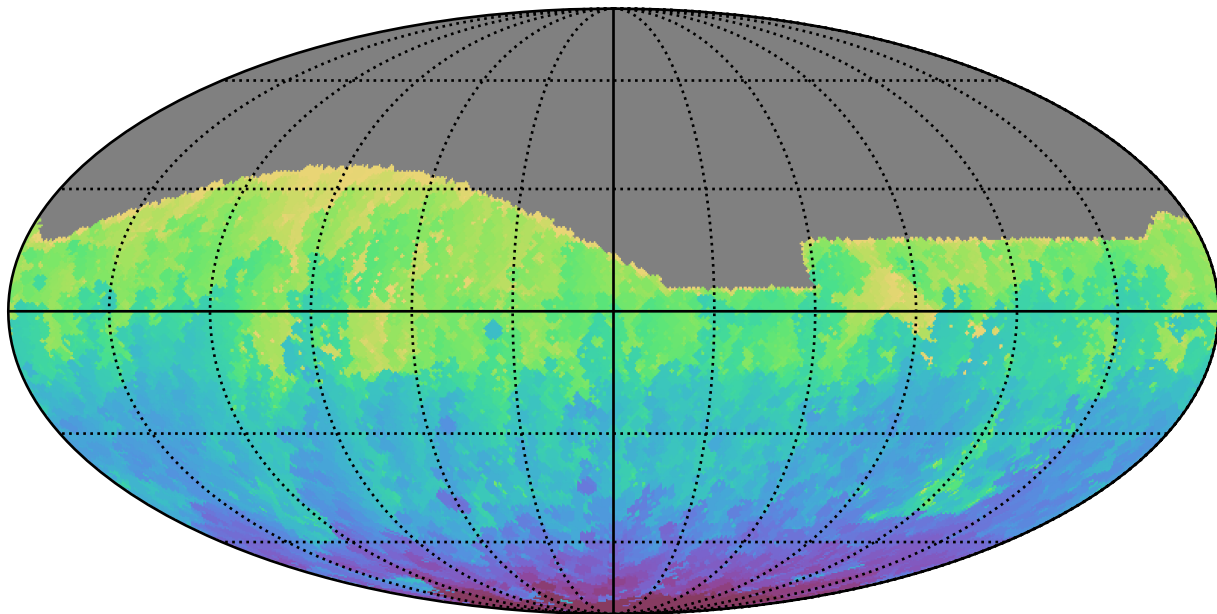
noroll_mjdp0_v3.4_10yrs All sky g band: Min HA
