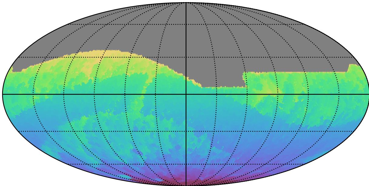
noroll_mjdp0_v3.4_10yrs All sky all bands: Min HA
