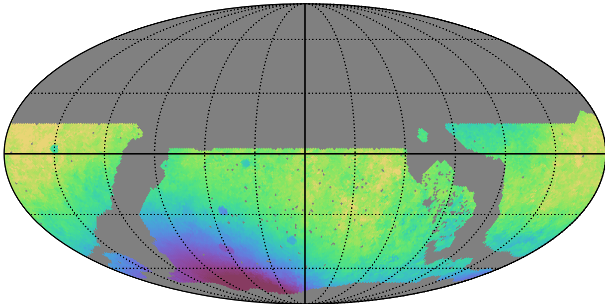
noroll_mjdp0_v3.4_10yrs WFD r band: Median solarElong
