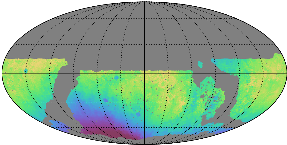
noroll_mjdp0_v3.4_10yrs WFD g band: Median solarElong
