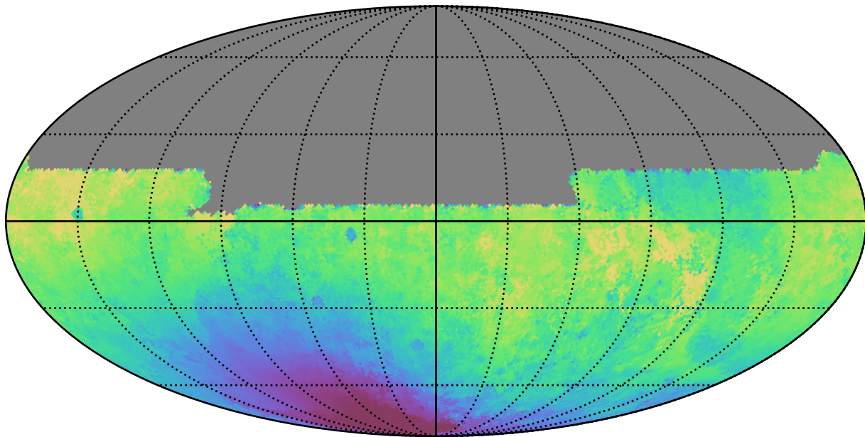
noroll_mjdp0_v3.4_10yrs All sky u band: Median solarElong
