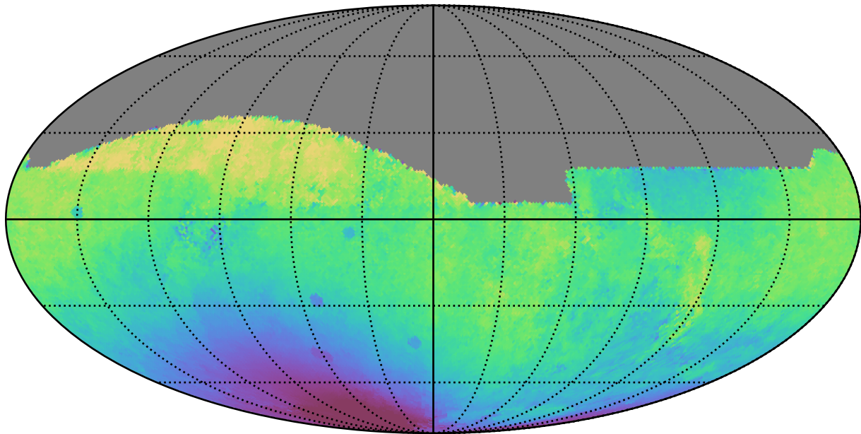
noroll_mjdp0_v3.4_10yrs All sky r band: Median solarElong
