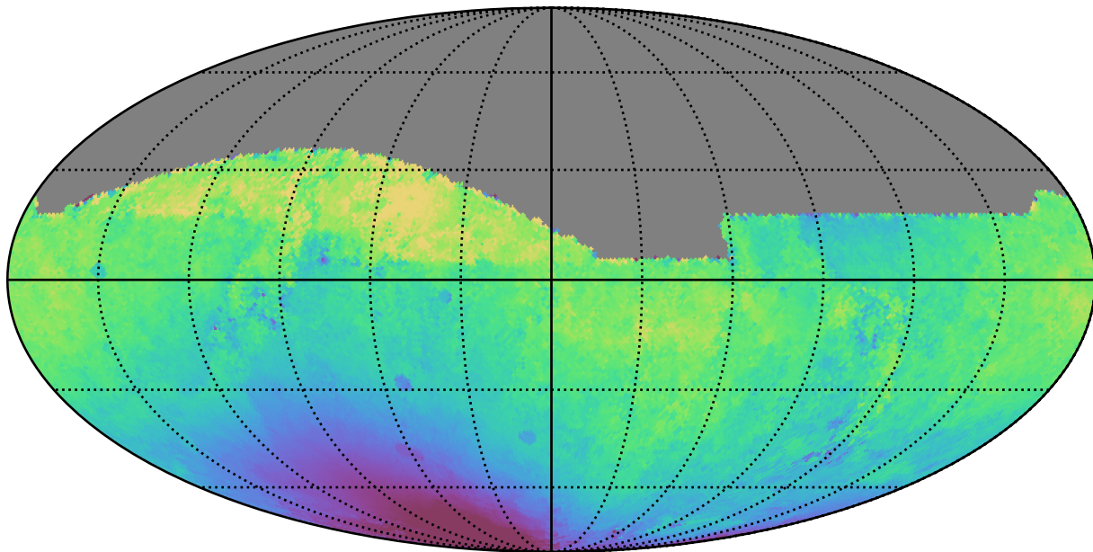
noroll_mjdp0_v3.4_10yrs All sky i band: Median solarElong
