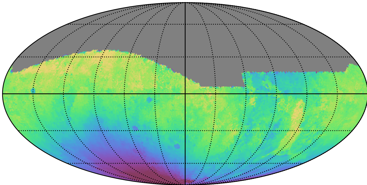
noroll_mjdp0_v3.4_10yrs All sky g band: Median solarElong
