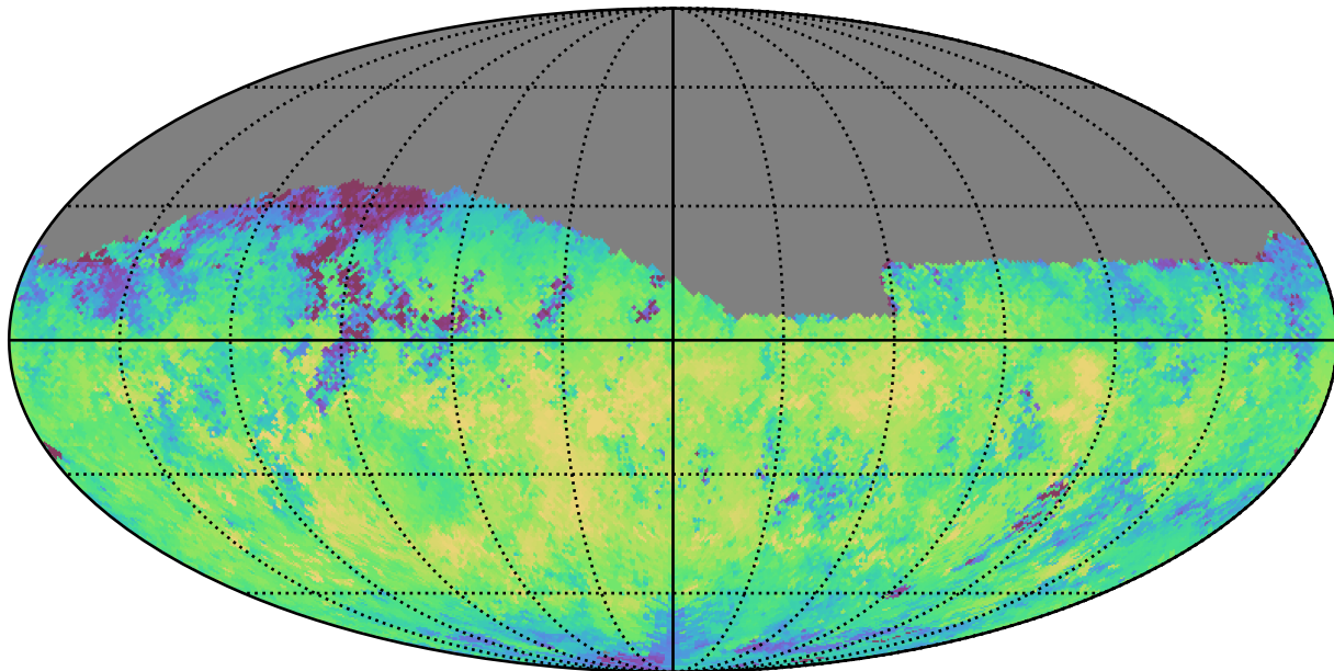
noroll_mjdp0_v3.4_10yrs Yr 1 z band: Median skyBrightness
