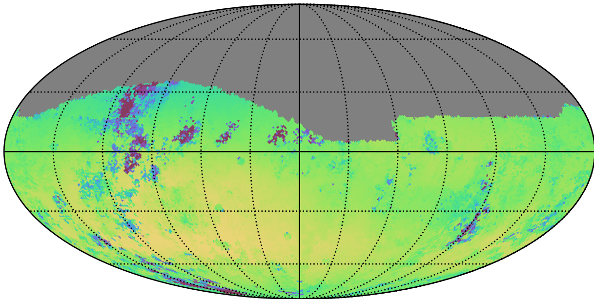
noroll_mjdp0_v3.4_10yrs Yr 1 r band: Median skyBrightness
