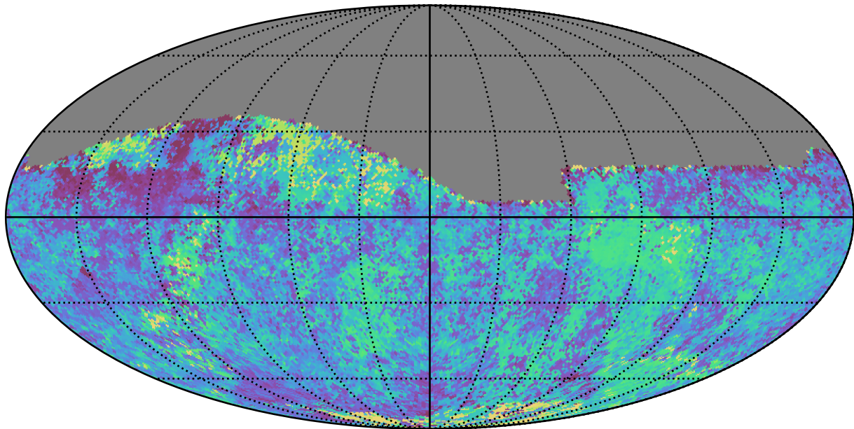
noroll_mjdp0_v3.4_10yrs Yr 1 all bands: Median skyBrightness
