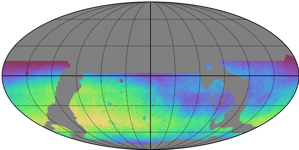
noroll_mjdp0_v3.4_10yrs WFD u band: Median skyBrightness
