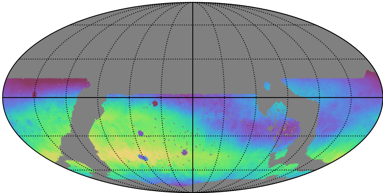
noroll_mjdp0_v3.4_10yrs WFD r band: Median skyBrightness
