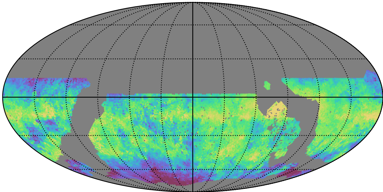
noroll_mjdp0_v3.4_10yrs WFD i band: Median skyBrightness
