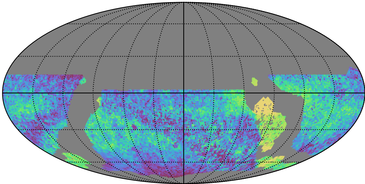
noroll_mjdp0_v3.4_10yrs WFD all bands: Median skyBrightness
