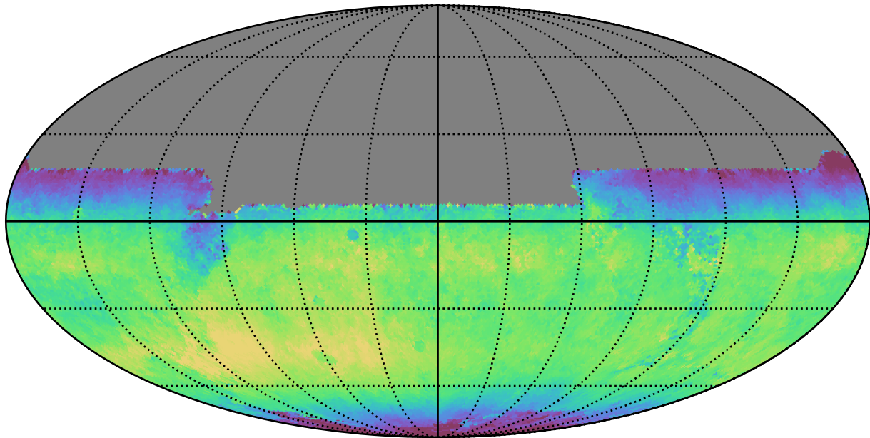
noroll_mjdp0_v3.4_10yrs All sky y band: Median skyBrightness
