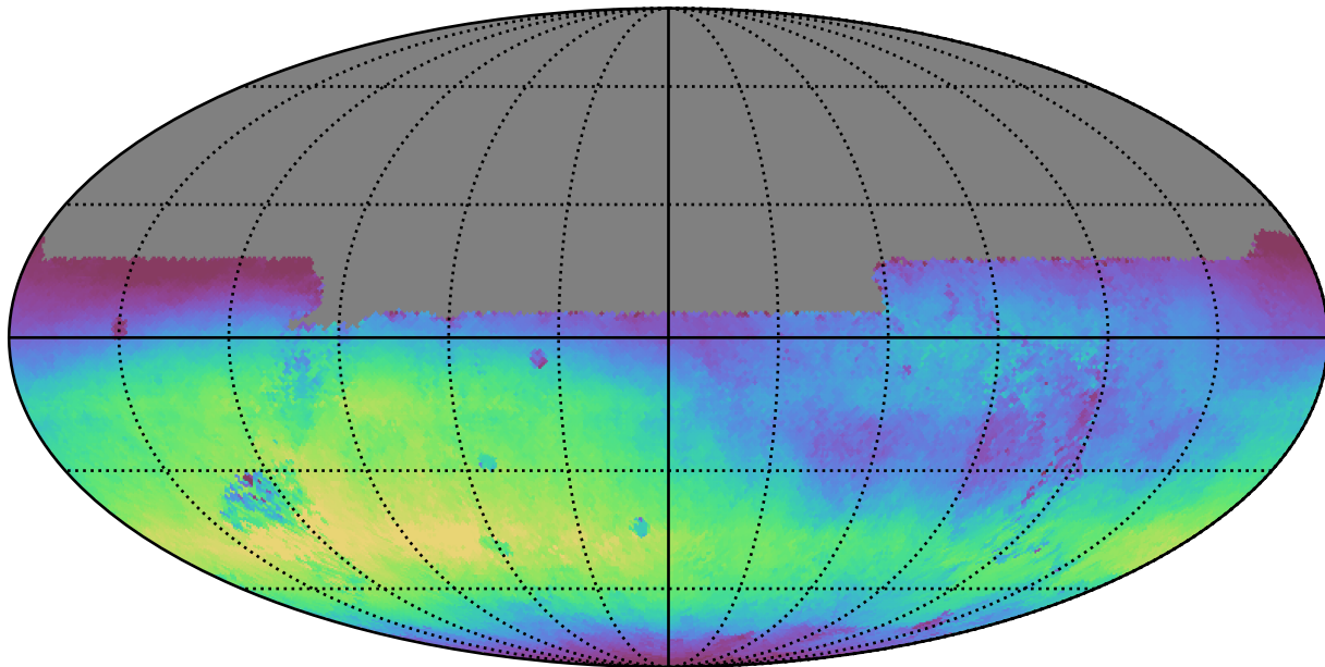
noroll_mjdp0_v3.4_10yrs All sky u band: Median skyBrightness
