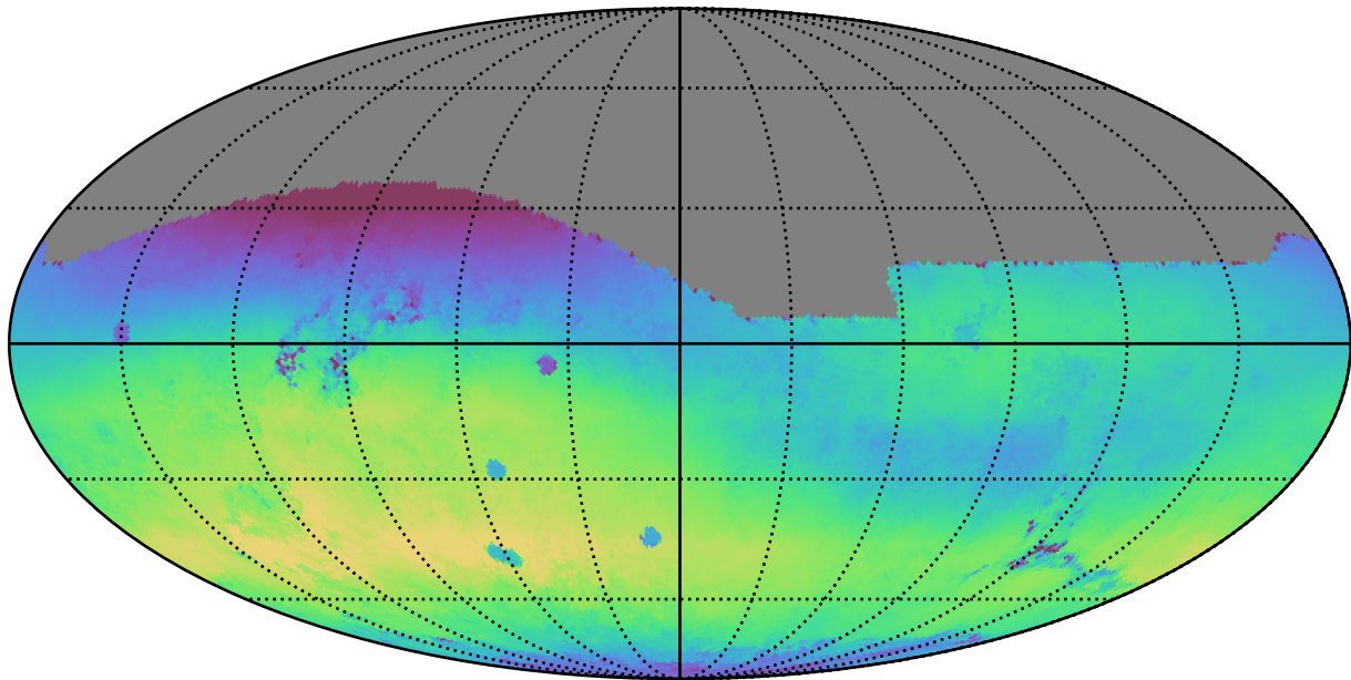
noroll_mjdp0_v3.4_10yrs All sky r band: Median skyBrightness
