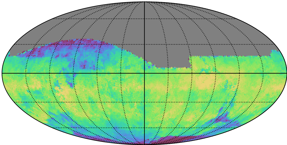
noroll_mjdp0_v3.4_10yrs All sky i band: Median skyBrightness
