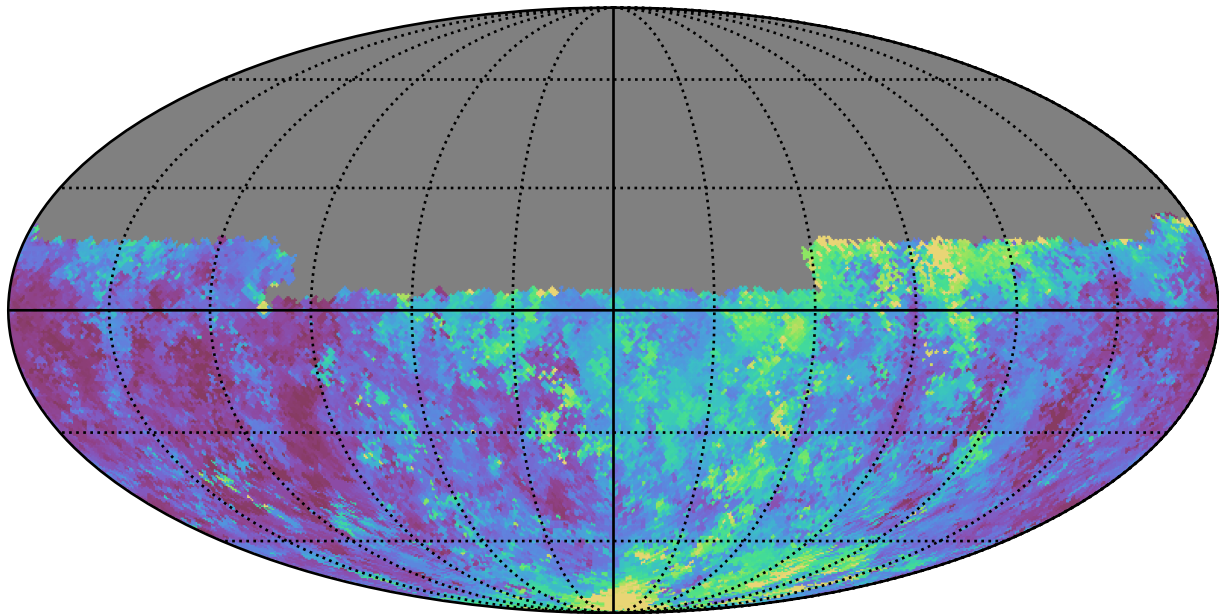
noroll_mjdp0_v3.4_10yrs Yr 1 u band: Median seeingGeom
