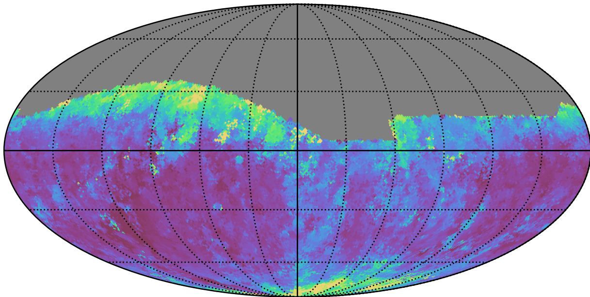
noroll_mjdp0_v3.4_10yrs Yr 1 r band: Median seeingGeom
