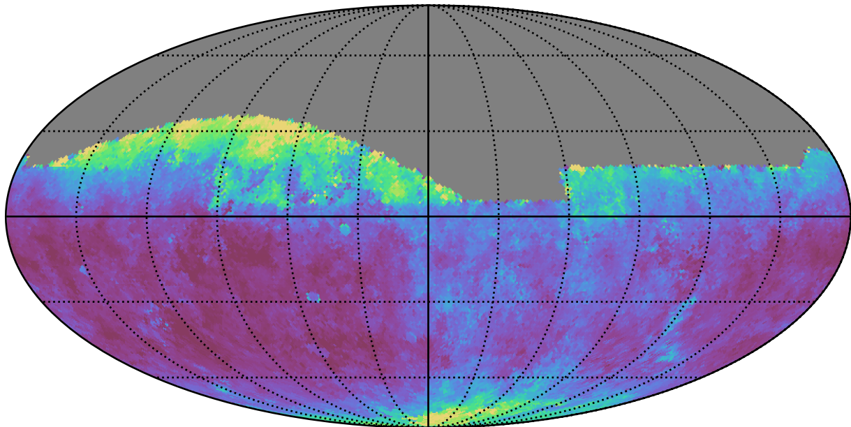
noroll_mjdp0_v3.4_10yrs Yr 1 all bands: Median seeingGeom
