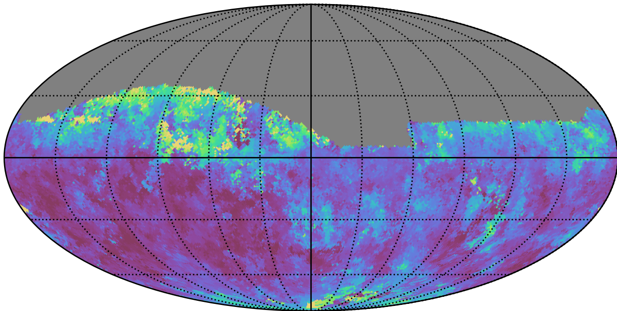
noroll_mjdp0_v3.4_10yrs Yr 1 z band: Median seeingEff
