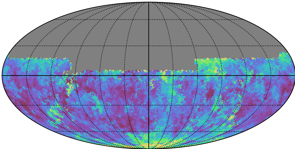
noroll_mjdp0_v3.4_10yrs Yr 1 y band: Median seeingEff
