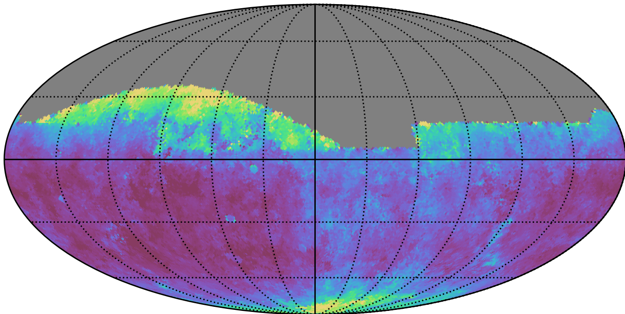
noroll_mjdp0_v3.4_10yrs Yr 1 all bands: Median seeingEff
