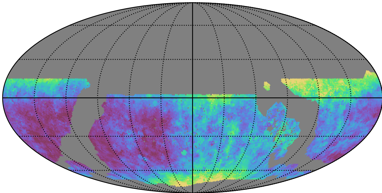
noroll_mjdp0_v3.4_10yrs WFD y band: Median seeingEff
