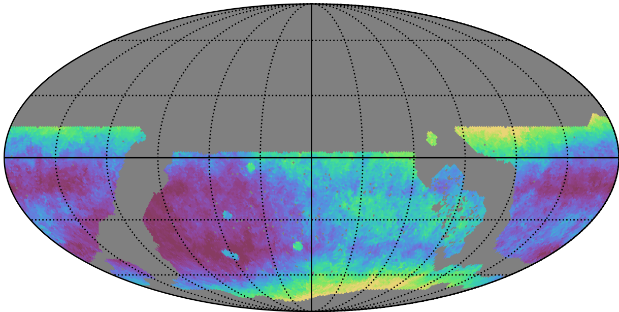
noroll_mjdp0_v3.4_10yrs WFD r band: Median seeingEff
