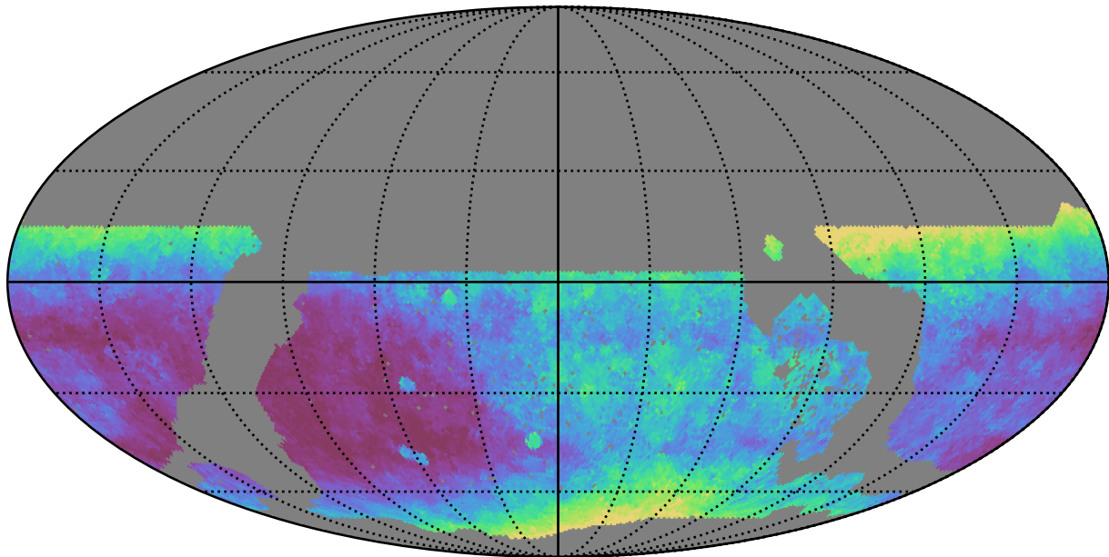
noroll_mjdp0_v3.4_10yrs WFD i band: Median seeingEff
