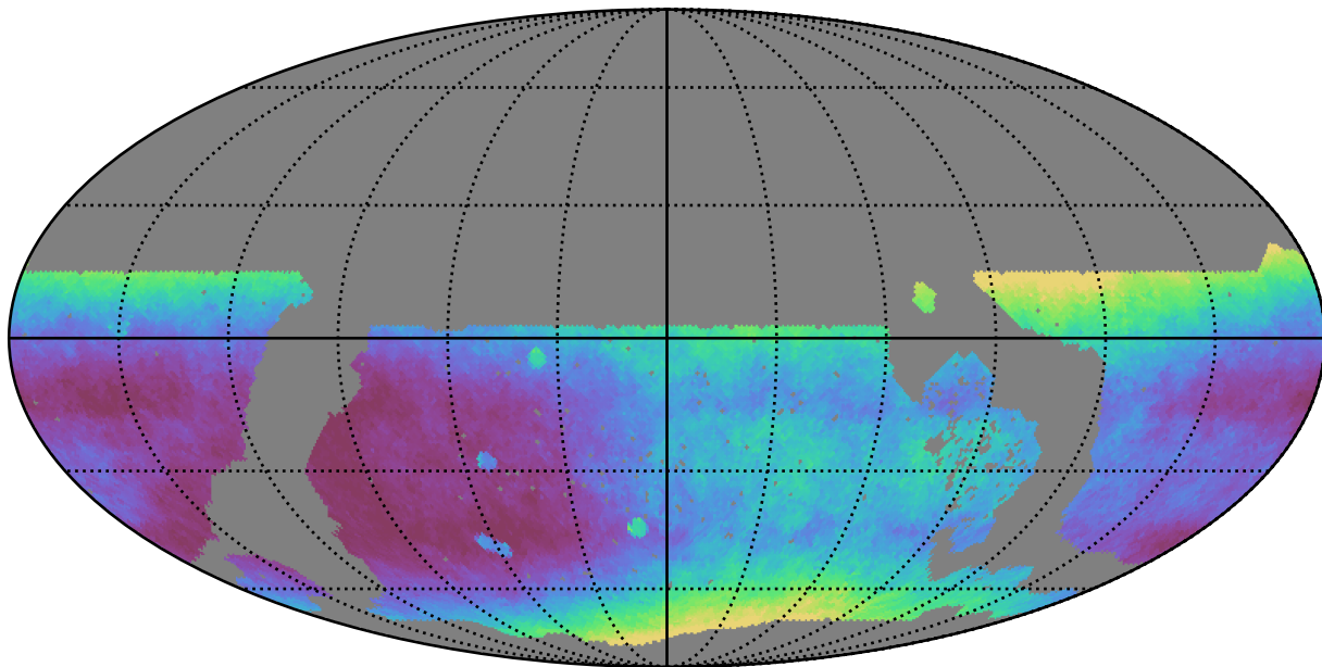
noroll_mjdp0_v3.4_10yrs WFD all bands: Median seeingEff
