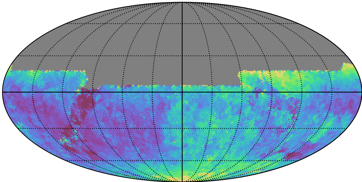
noroll_mjdp0_v3.4_10yrs All sky u band: Median seeingEff
