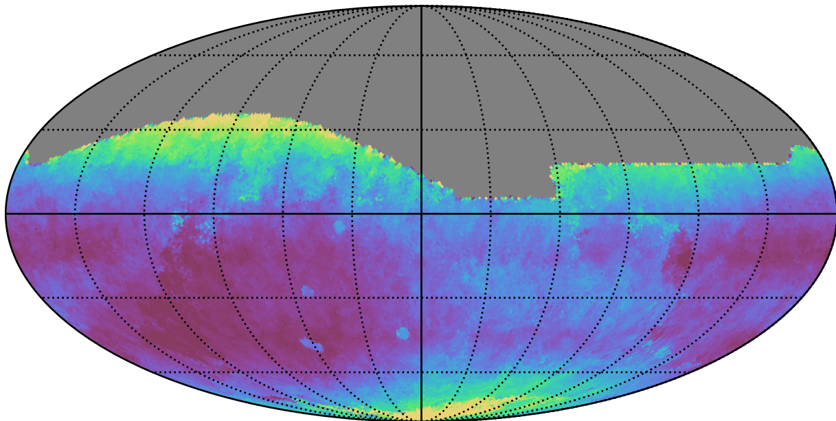
noroll_mjdp0_v3.4_10yrs All sky r band: Median seeingEff
