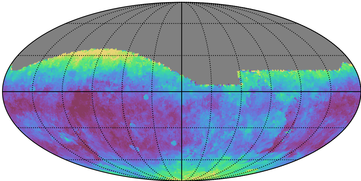
noroll_mjdp0_v3.4_10yrs All sky g band: Median seeingEff
