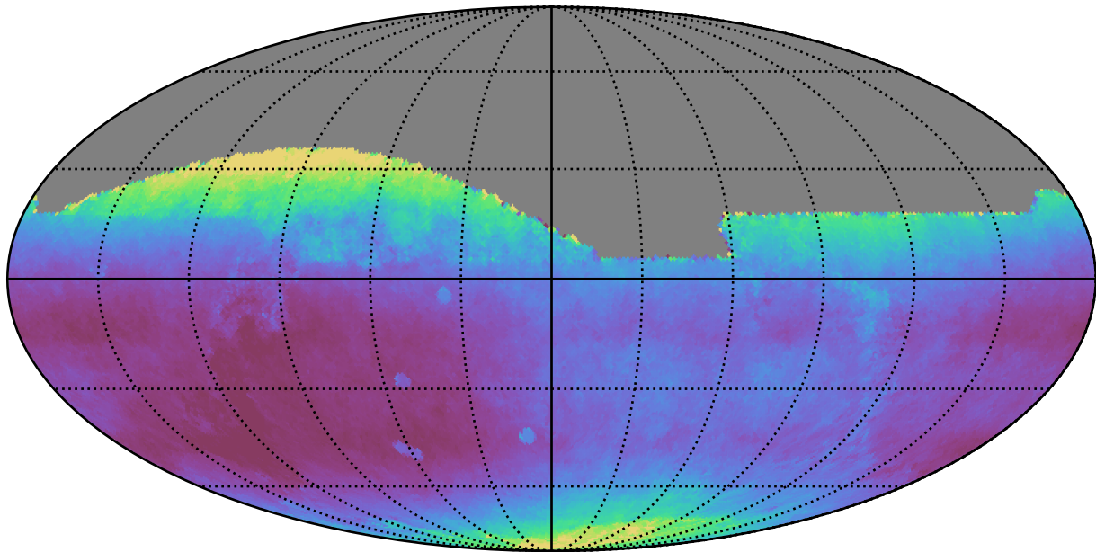
noroll_mjdp0_v3.4_10yrs All sky all bands: Median seeingEff
