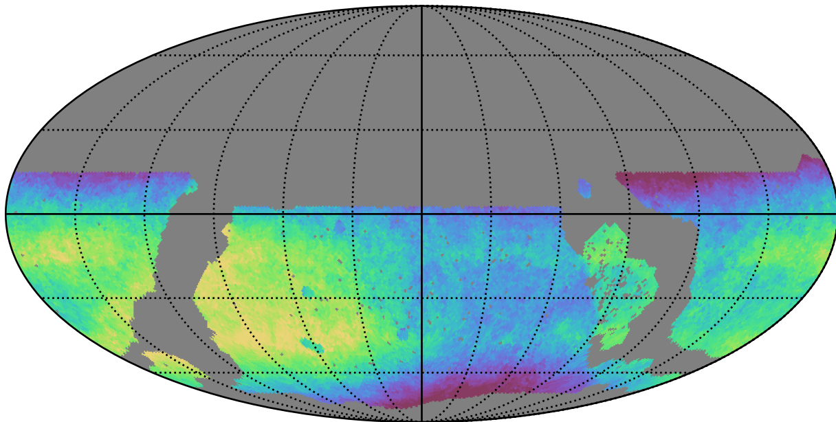
noroll_mjdp0_v3.4_10yrs WFD all bands: Median saturation_mag
